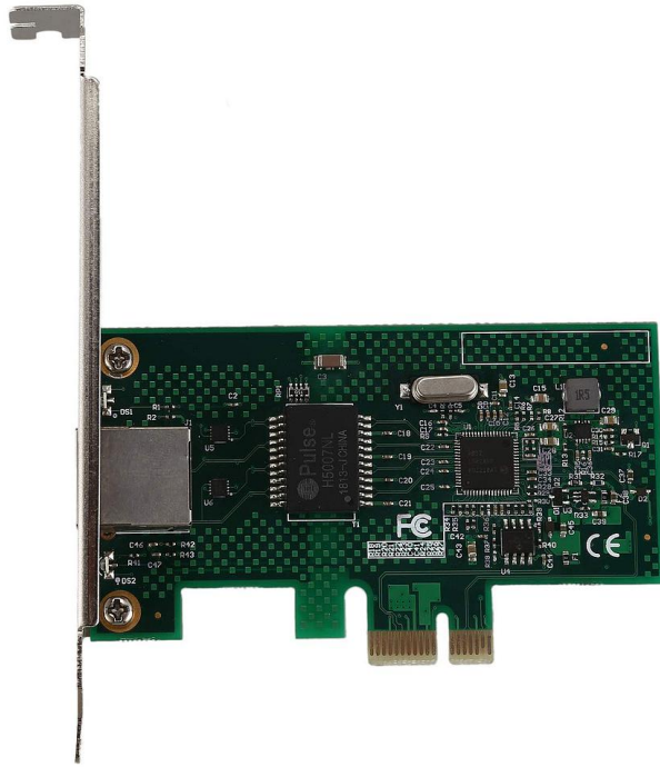
Broadcom BCM5751 PCI Express Lan Card
